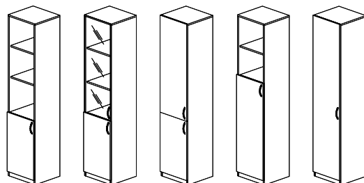
В.ПР-2 650x300x16
